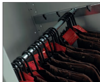
Garment hanging - Adjustable rails and brackets. Three rail slot positions in 300, 400, 450 & 500mm deep brackets and 5 rail slot positions in 600 & 750mm.
